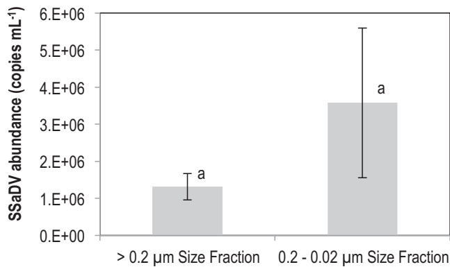
Fig. 8. Viral abundance in particle (i.e., >0.2 μm) and viroplankton (0.2–0.02 μm) size fractions of water collected at field sites, experimental incubations, and public aquaria. Viral abundance was determined by qPCR targeting the VP4 gene of the SSaDV genome. Means were not significantly different.
